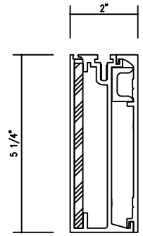
D2 1 DETAIL BOX PERIMETER WITH REINFORCEMENT BP253/BP252
