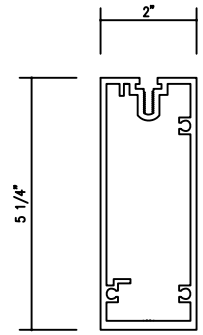
D3 1 DETAIL SOLID STACK JOIST SJ253
