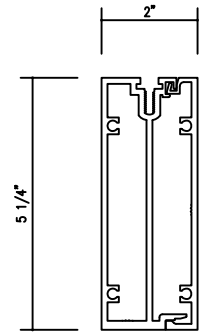
D5 1 DETAIL STACK JOIST SJ254/SJ252
