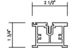
D6 1 DETAIL ROOF /SHALLOW JOIST RJ251
