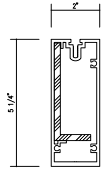
D4 1 DETAIL SOLID STACK JOIST WITH REINFORCEMENT SJ253
